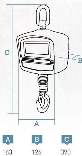
Dimensions DATA IN mm
